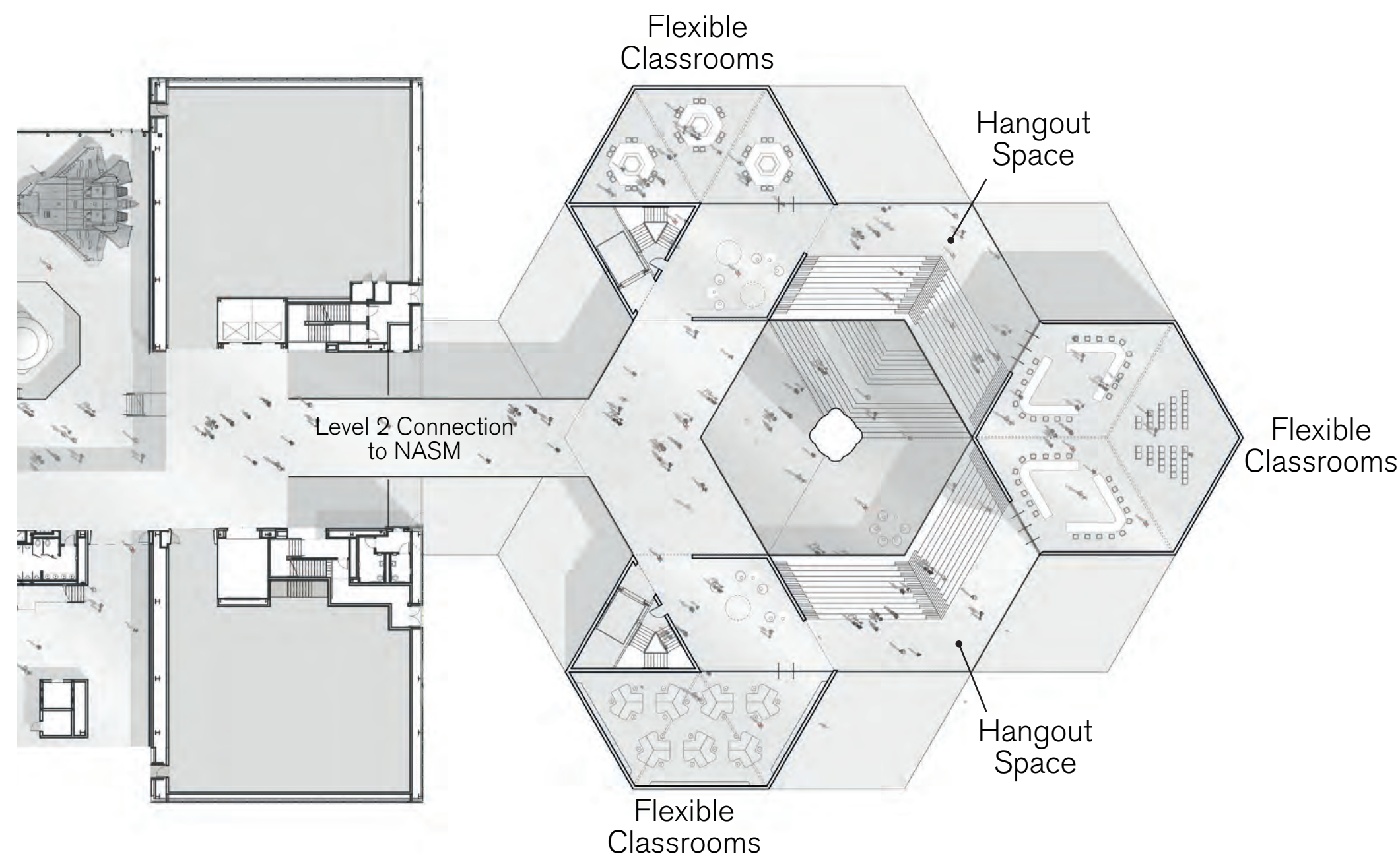
Level 2 Plan - Learning Center
