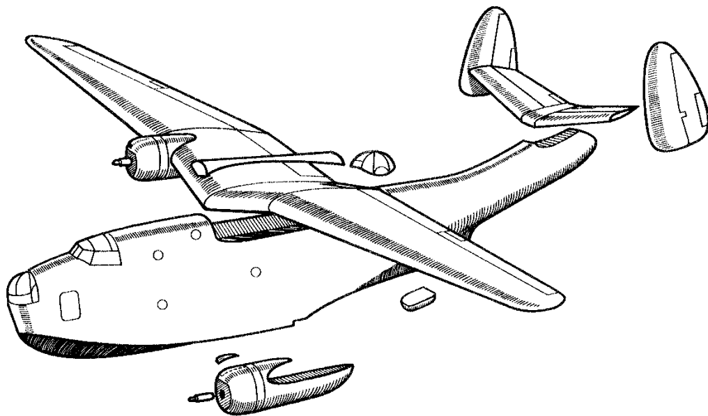
Exploded View of Martin PBM-1 Recognition Model (Code B-2)
