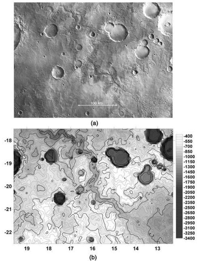
Figure 3. The relationship between fluvial dissection and topography in the vicinity of Loire Valles. (A) Regional mosaic of Viking images from orbit F615A centered at about 20^\circ lat., 15^\circ long. (B) Topography of the same region based upon MOLA data released through 30 August 1999. The contour interval is 100 m and the scale in kilometers.
