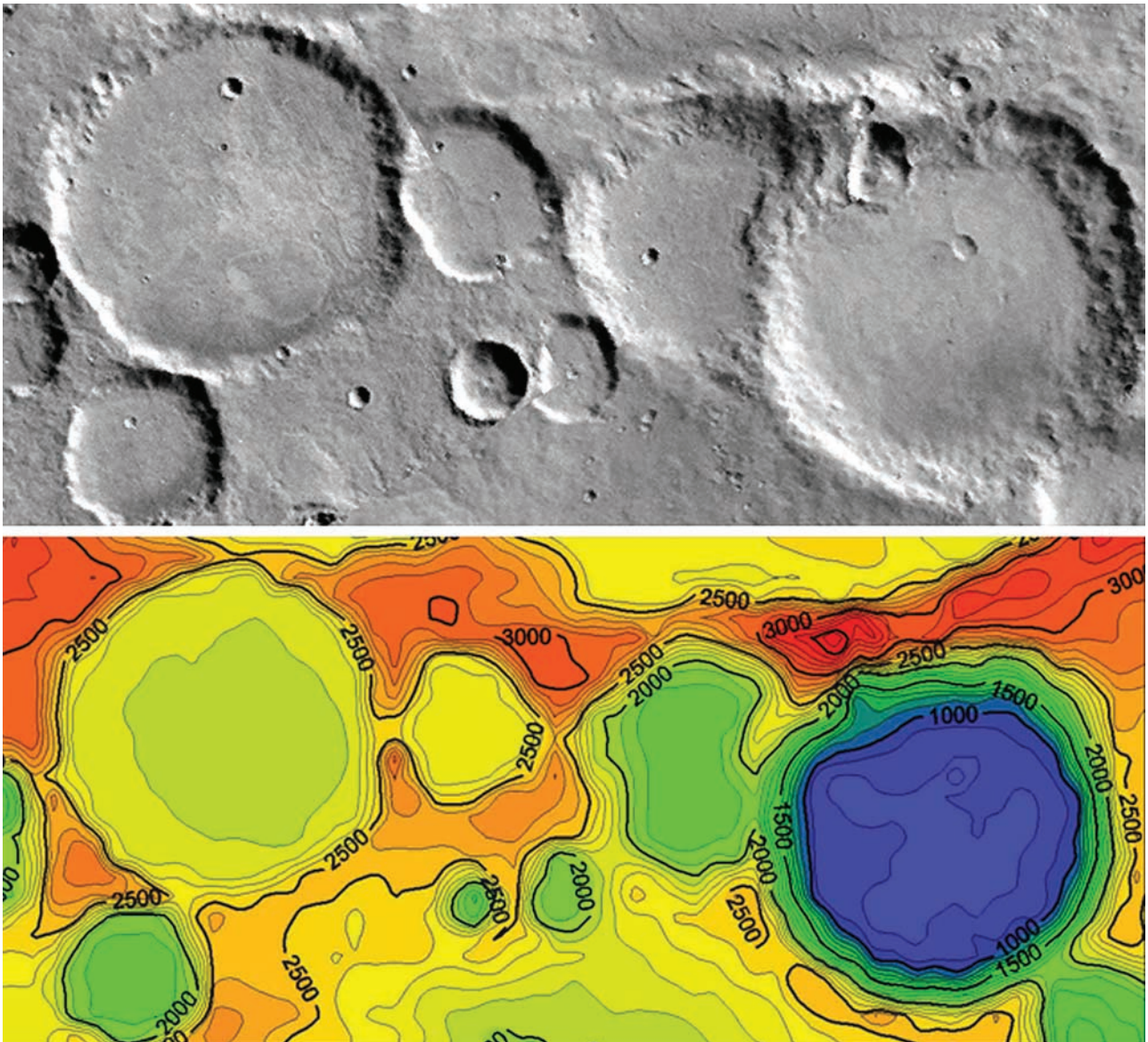
Figure 8. Massive erosion and infilling are evidenced by this group of craters on the border of the Sinus Sabaeus quadrangle centered at 21^{\circ}, 317^{\circ} . (A) The two largest craters are both 55 km in diameter and have undergone appreciable modification. (B) However, MOLA data show that the western crater has been infilled by perhaps as much as 1 km of material. Either it has experience extensive backwasting or sediments were transported from the surrounding terrain. It is unlikely volcanic infilling has take place since such deposits should fill surrounding craters to the same level [Howard, 1999; Howard and Craddock, 2000].
