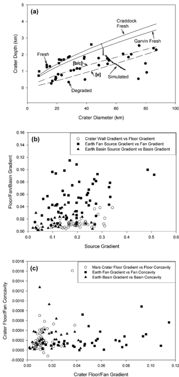
Figure 9. (opposite) Geometric properties of Martian craters and terrestrial fan and basin deposits. (A) Plot of crater depth (from rim to crater floor) versus crater diameter for fresh and degraded craters. Measurements made from MOLA data in the Margaritifer Sinus and Iapygia regions of Mars. Summary depth/diameter relationships for relatively unmodified craters are from Craddock et al. [1997] “Craddock Fresh,” based upon photogrammetric techniques and from MOLA DEM data “Garvin Fresh” from Garvin et al. [2000]. Also shown are summary relationships for moderately degraded craters of class B and C “[b/c]” and for highly degraded craters “[e]” from Craddock et al. [1997]. A plot of the temporal change of crater depth and crater diameter is shown for simulated dissection of a 50-km crater (see Figure 11). (B) Plot showing the relationship between the average gradient of the inward-sloping surfaces of degraded crater floors (e.g., Figure 10) and the average gradient of the corresponding interior crater rim, from measurements made from MOLA profiles. Also shown are the gradients of alluvial fans in the Southwestern United States plotted against the average gradient of the source mountains (from mountain crest to fan head), as well as a similar relationship for lower-gradient alluvial basins in the United States. The terrestrial data is from topographic maps and 1:250,000 DEM data. (C) The relationship between the concavity of Martian degraded crater floors and the gradient of the crater floor, as well as corresponding data from terrestrial fans and basins. (D) The total relief of Martian degraded crater floors (from the base of the interior crater wall to the center of the crater) is plotted versus crater diameter.
