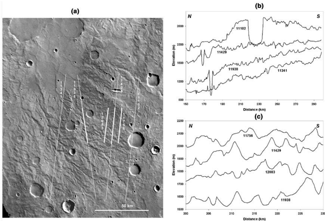
Figure 15. A dissected regional slope centered at 10.5^{\circ} lat., 245^{\circ} long. (A) Mosaic of images from Viking Orbiter F629A showing selected MOLA tracks, identified by orbit number. (B) Topography derived from MOLA profiles. Profile 11938 is displaced vertically by +200 m, 11429 by +400 m and 11102 by +800 m. Vertical exaggeration about 44X. (C) Detailed profiles showing morphometric attributes of some valley networks. Profiles 11756 and 11429 are displaced vertically by +100 m. Vertical exaggeration about 28X.
