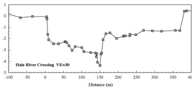
Figure 4. The flat floor morphology associated with many valley networks is not necessarily diagnostic of groundwater sapping. A rectangular (or “U-shaped”) cross-section is characteristic of many terrestrial rivers where the channel is in equilibrium between discharge, slope, and channel boundary conditions. Ephemeral rivers in central Australia, for example, are fed primarily by surface runoff. Streams conform to a flat floor morphology to adjust for the high sediment volumes carried in bed load (>35%). Shear stresses are high over the bed and flow velocities are low along the erodible banks [Mabbutt, 1977, p. 160]. Not only do such streams have a morphology similar to many valley networks, but their drainage densities are typically low due to the high infiltration capacity of the soil. This results in a stream with a rectangular profile, such as the Hale River depicted here.
