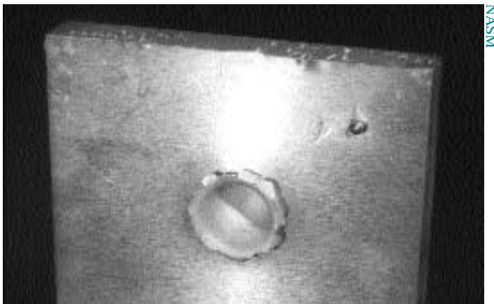
This block of aluminum shows the damage caused by a BB-sized object moving about 6,000 m/s (13,400 mph), which is slower than orbiting objects move. (Crater shown actual size.)
